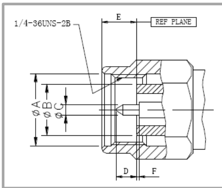
2.92mm Male
