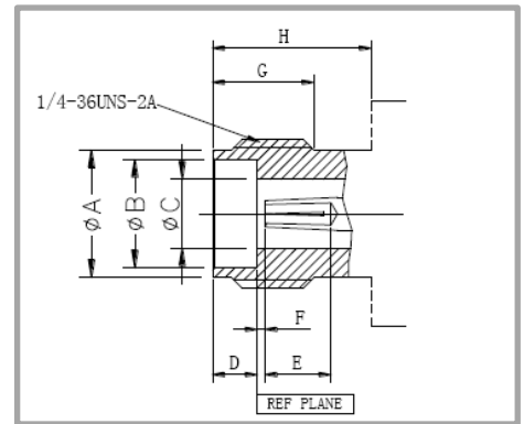
2.92mm Female
