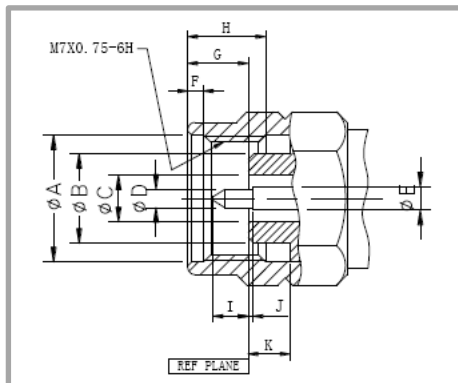
2.4mm Male
