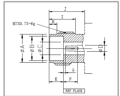
2.4mm Female
