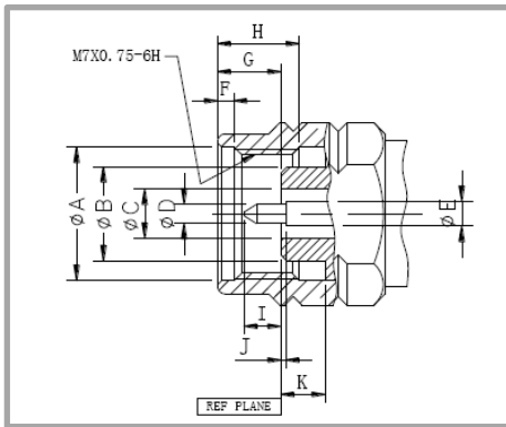
1.85mm Male
