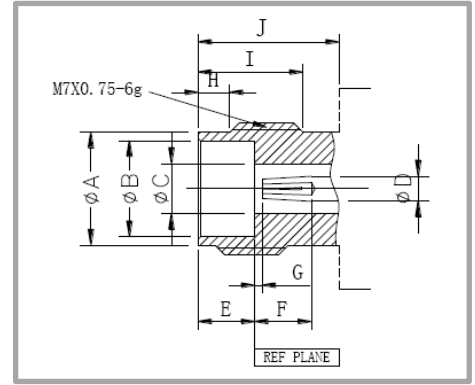
1.85mm Female
